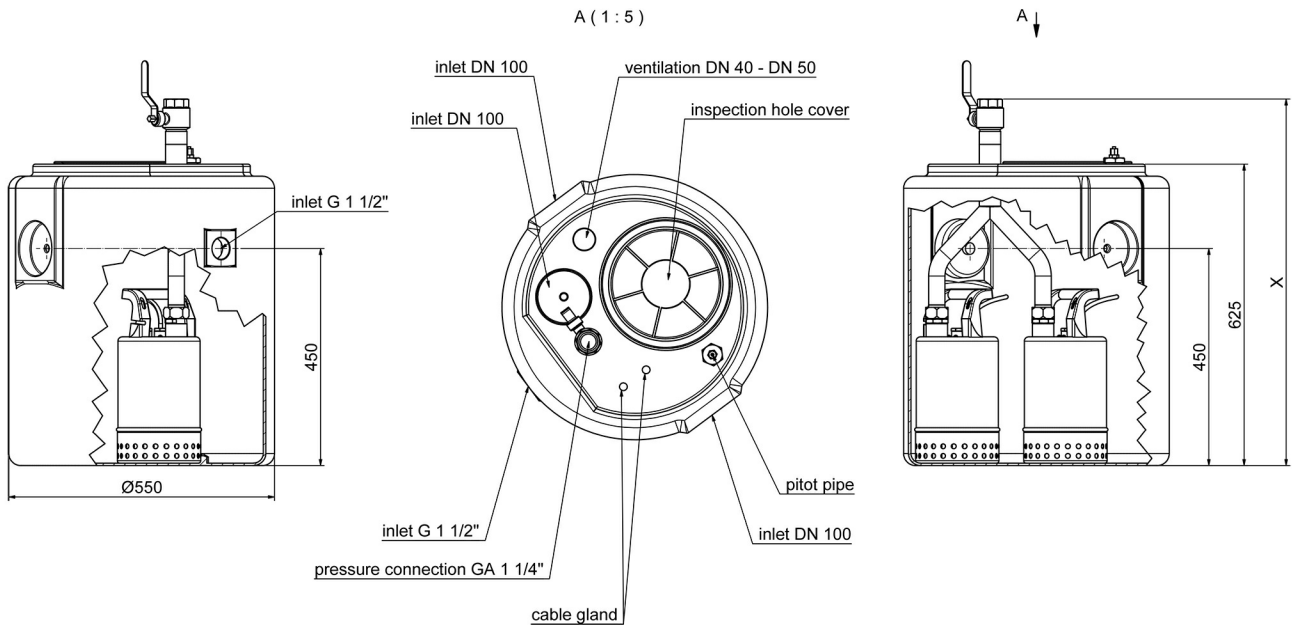
duplex unit
